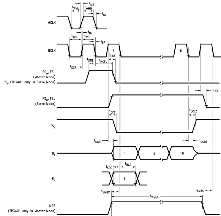
FIGURE 10. B Channel Interface Timing Details
